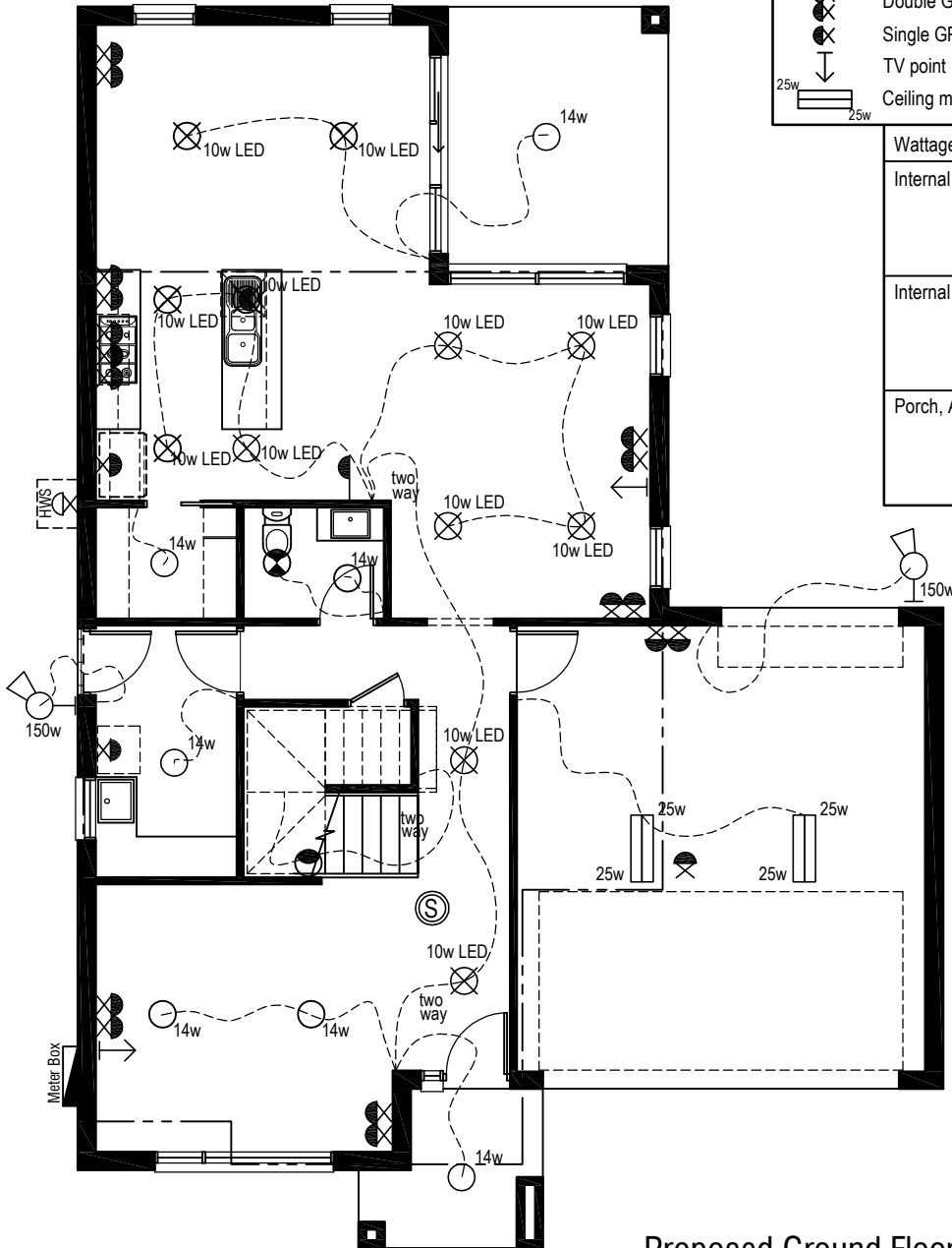
Proposed Ground Floor Electrical Plan
