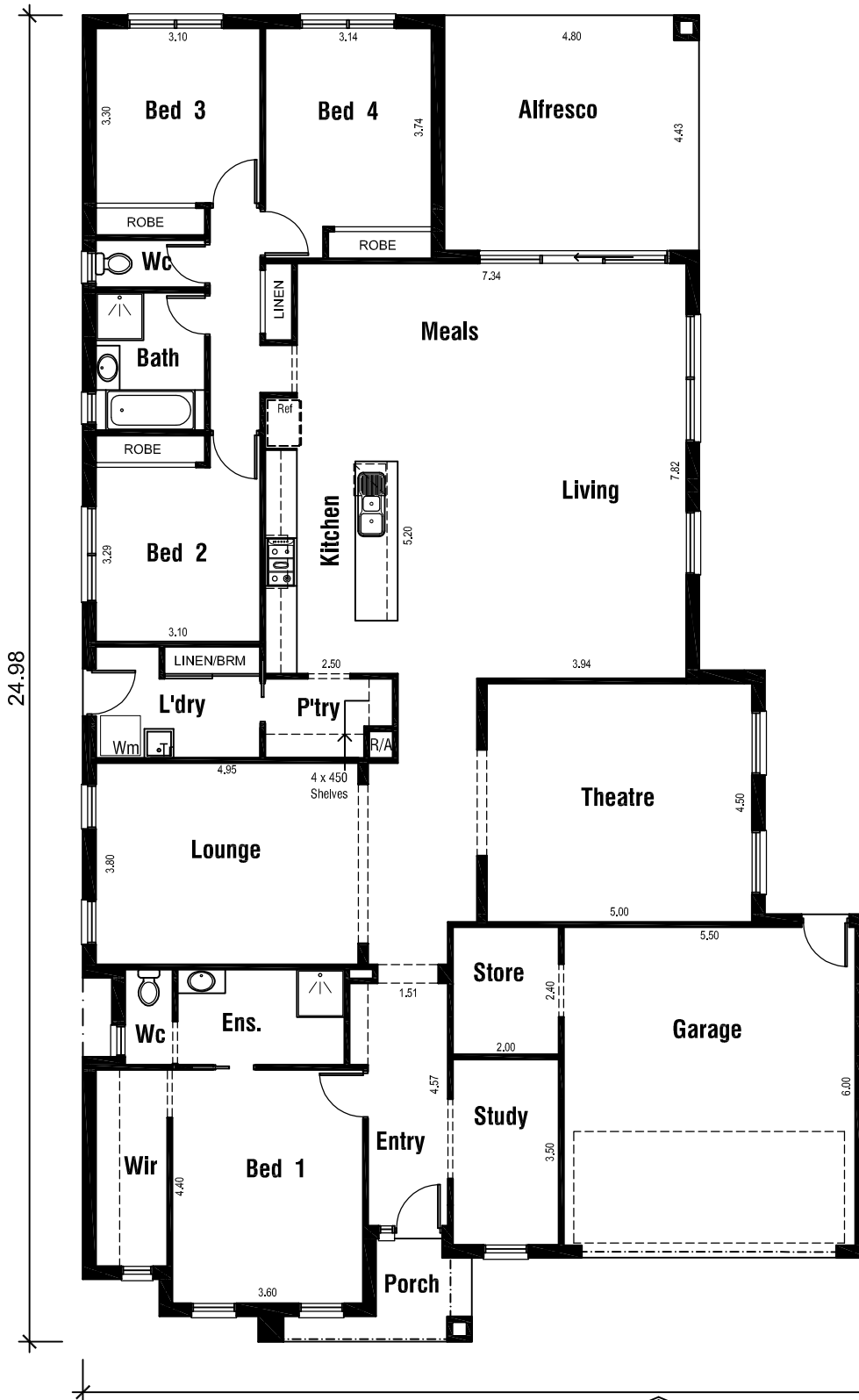
Floor Plan
