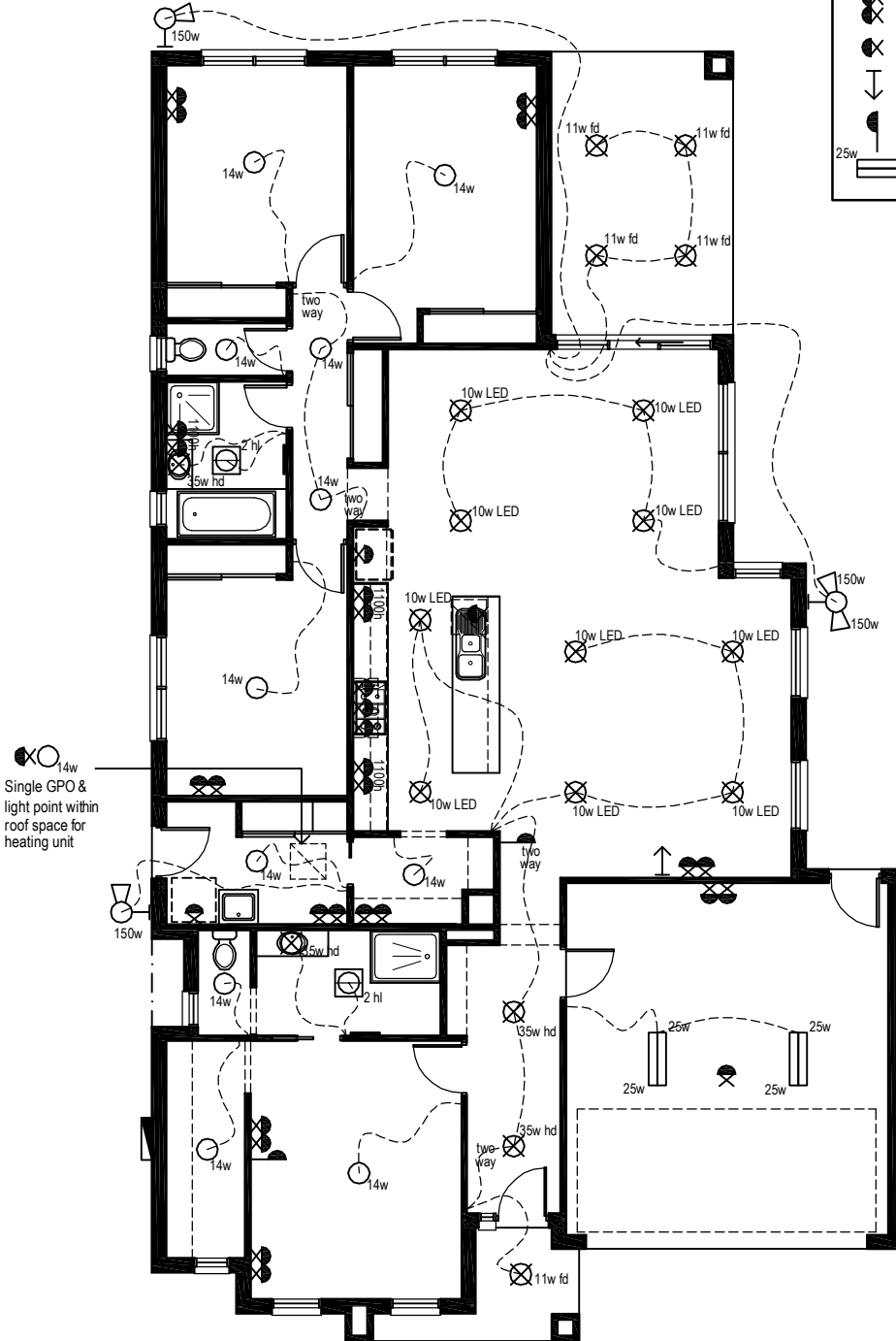
Proposed First Floor Electrical Plan
